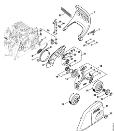
Hand guard, Chain brake
