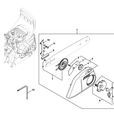
Quick chain tensioner
