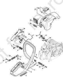
Handle frame, Shroud
