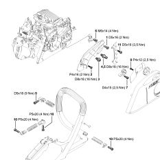
Tightening torques
