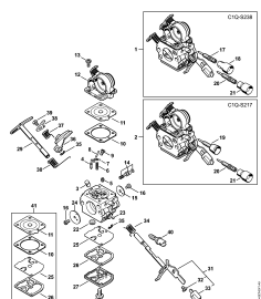
Carburetor C1Q-S238, C1Q-S217
