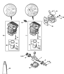
Cylinder, Muffler
