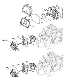
Air filter, Manifold
