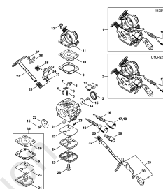
Carburetor 1139/29; C1Q-S270
