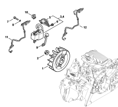
Ignition system
