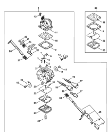
Carburetor C1Q-S123
